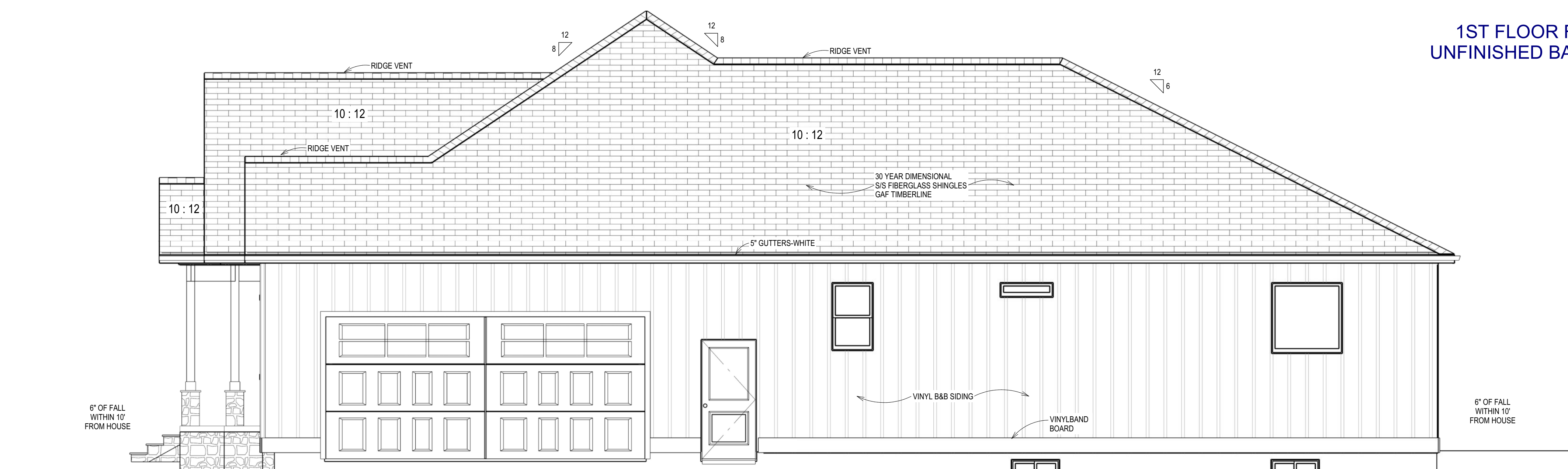
Exterior Elevation Right
