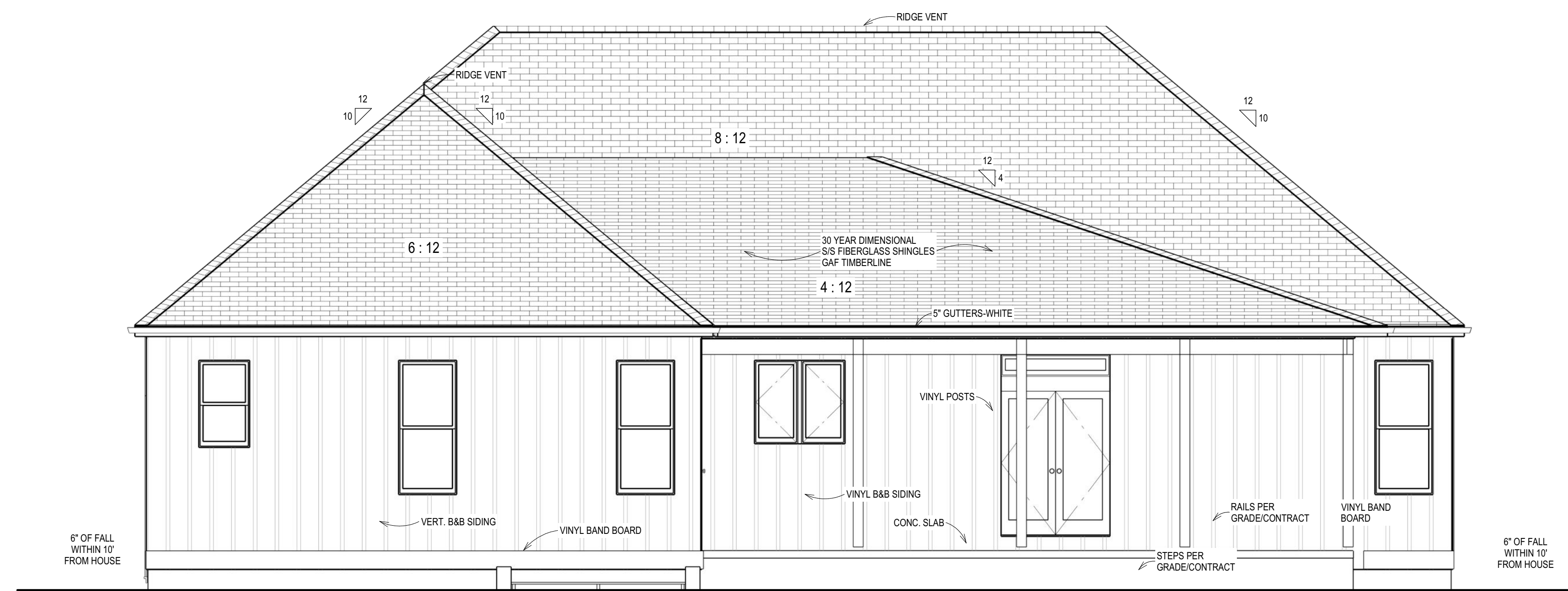
Exterior Elevation Back
