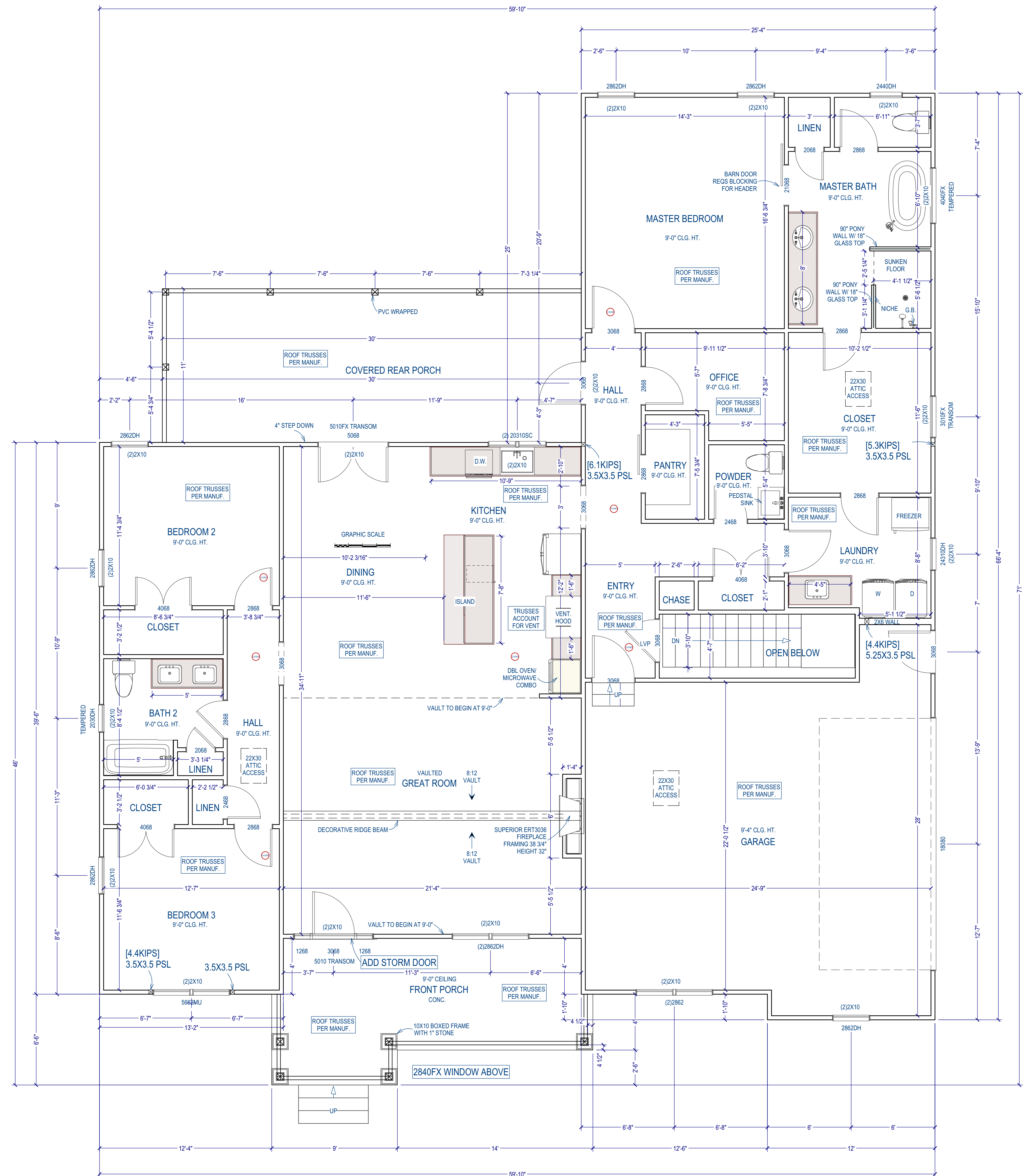
1ST FLOOR PLAN FINISHED=2,295 SQFT GARAGE=623 SQFT PORCHES=530 SQFT WINDOW DESIGNATION= ROUGH OPENING
