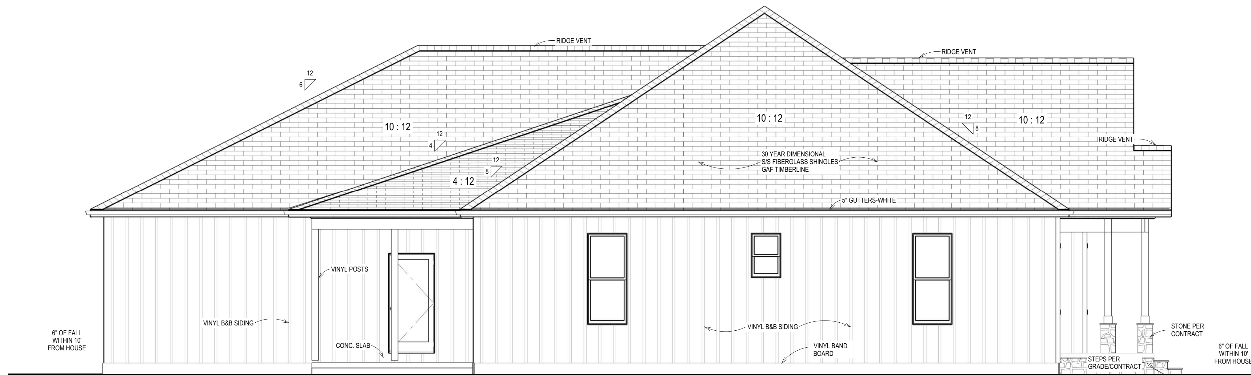
Exterior Elevation Left
